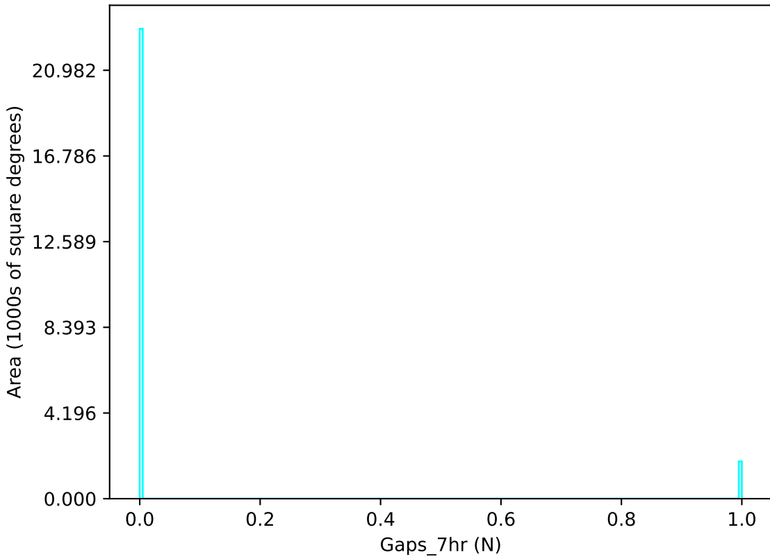
weather_cloudso6v3.4_10yrs u band: Gaps_7hr
