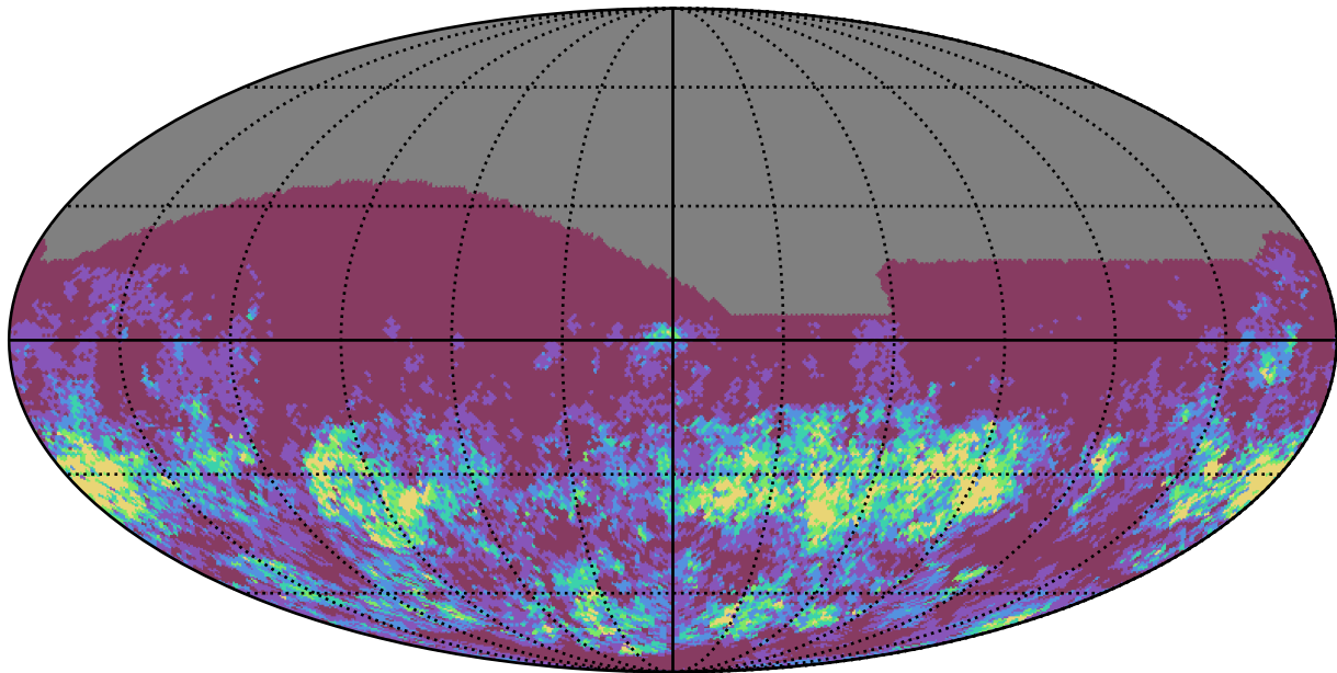
weather_cloudso6v3.4_10yrs r band: Gaps_7hr
