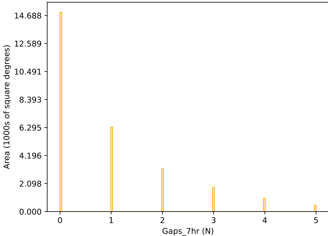
weather_cloudso6v3.4_10yrs r band: Gaps_7hr
