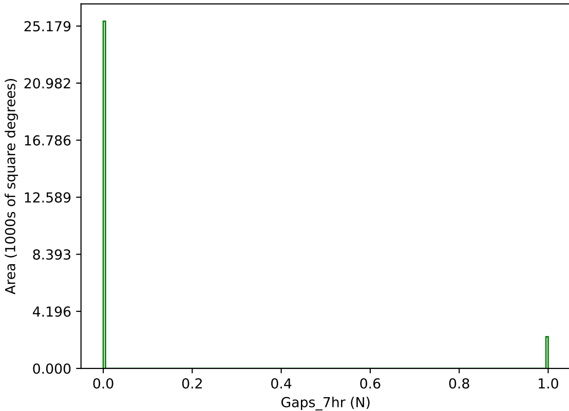
weather_cloudso6v3.4_10yrs g band: Gaps_7hr
