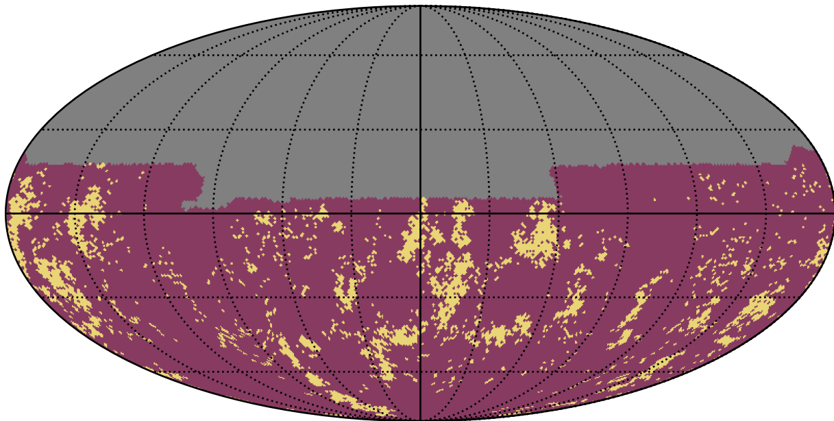
weather_cloudso6v3.4_10yrs u band: Gaps_3hr
