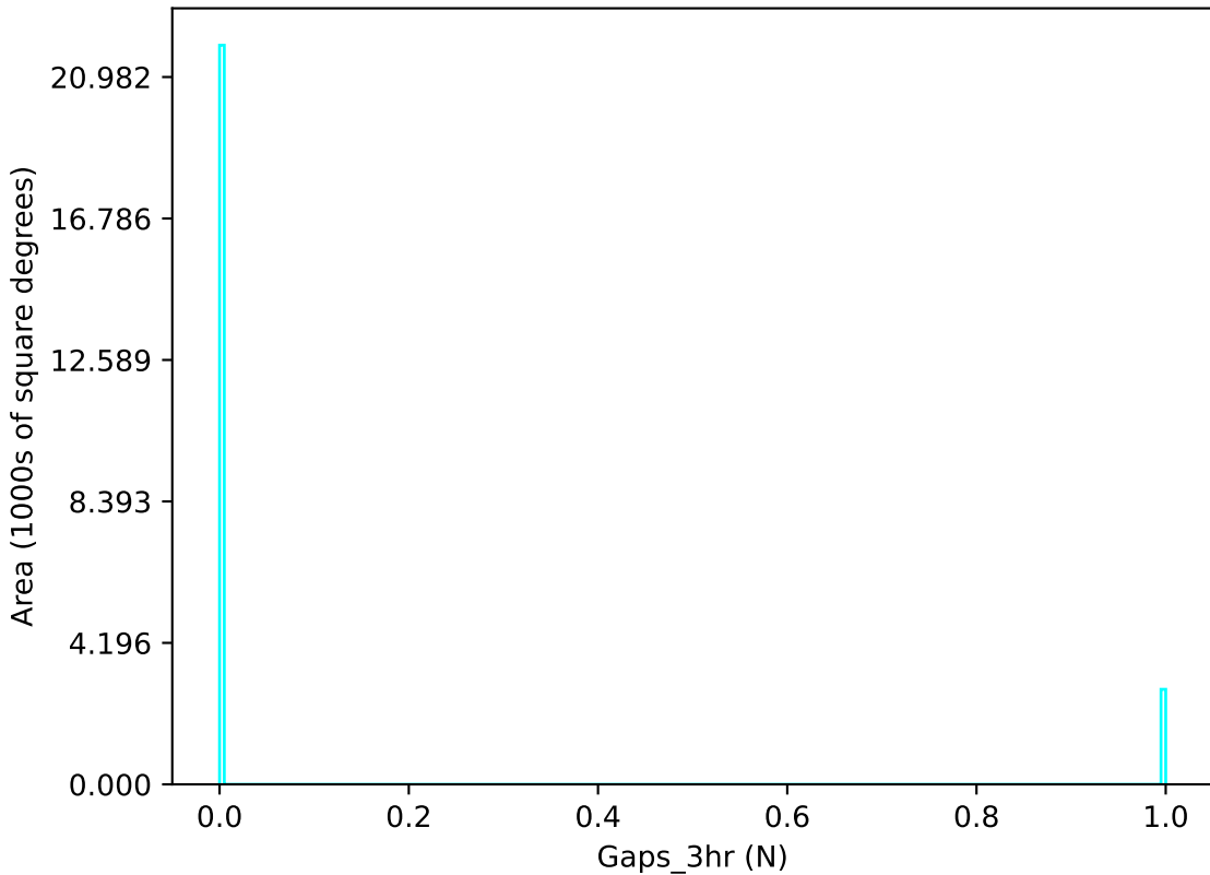
weather_cloudso6v3.4_10yrs u band: Gaps_3hr
