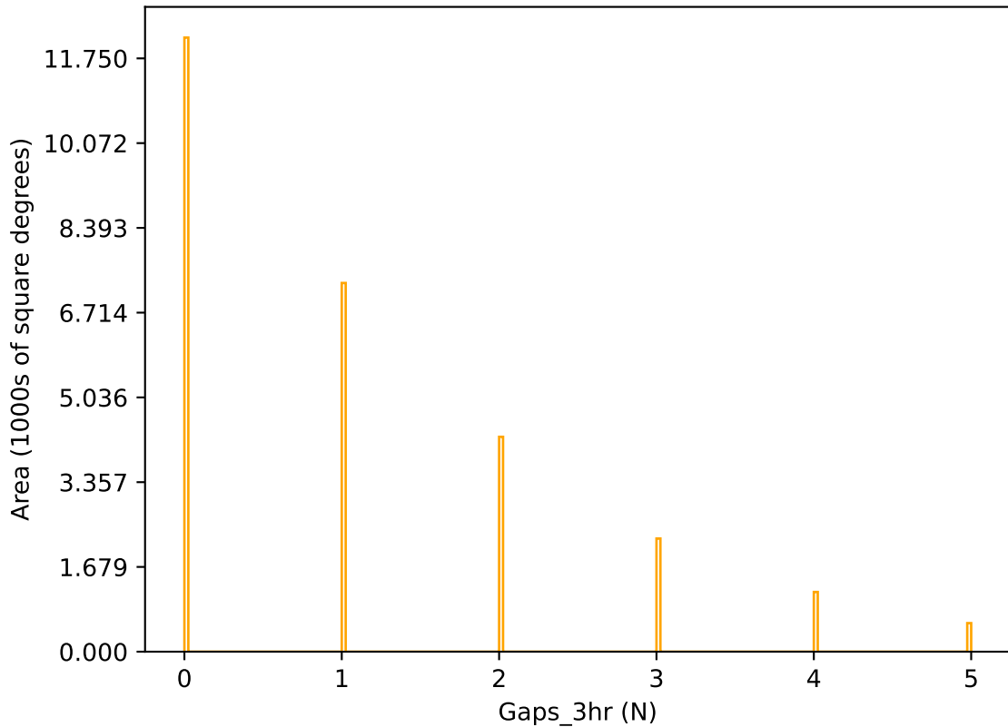
weather_cloudso6v3.4_10yrs r band: Gaps_3hr
