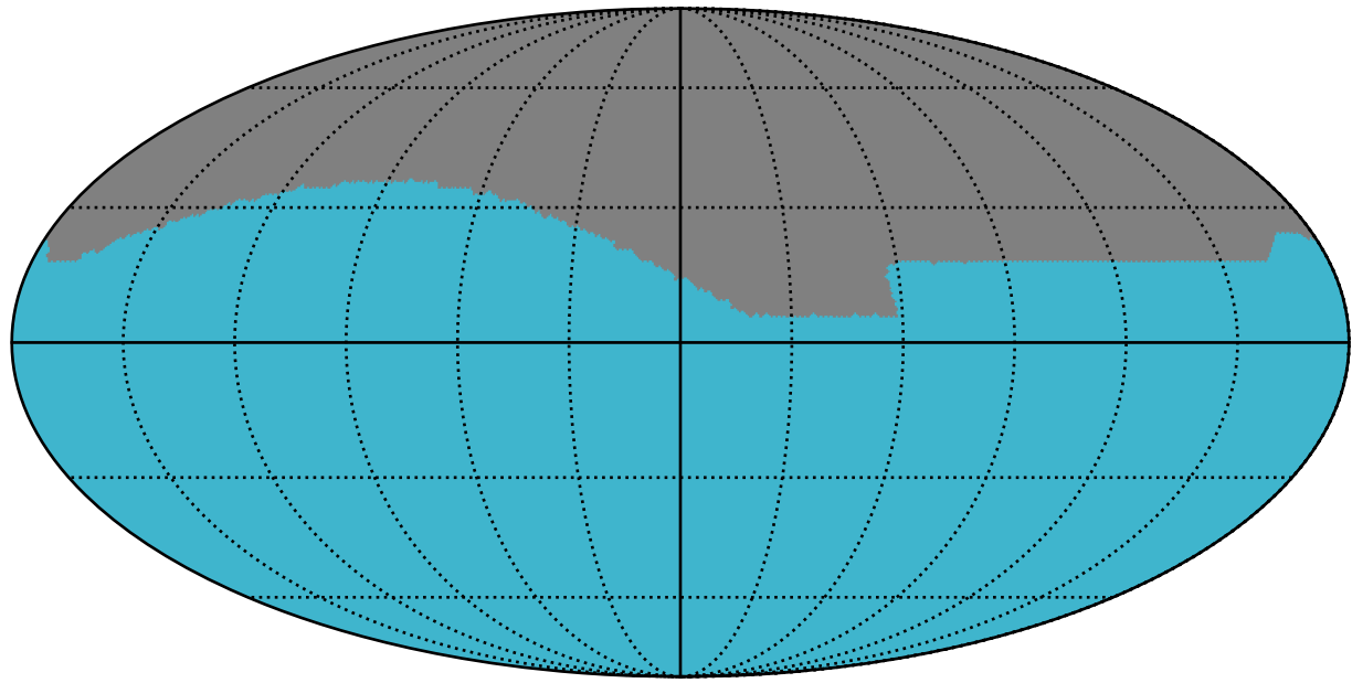
weather_cloudso6v3.4_10yrs : GalplaneFootprintMetric_xray_binaries_map_Tau_2_0
