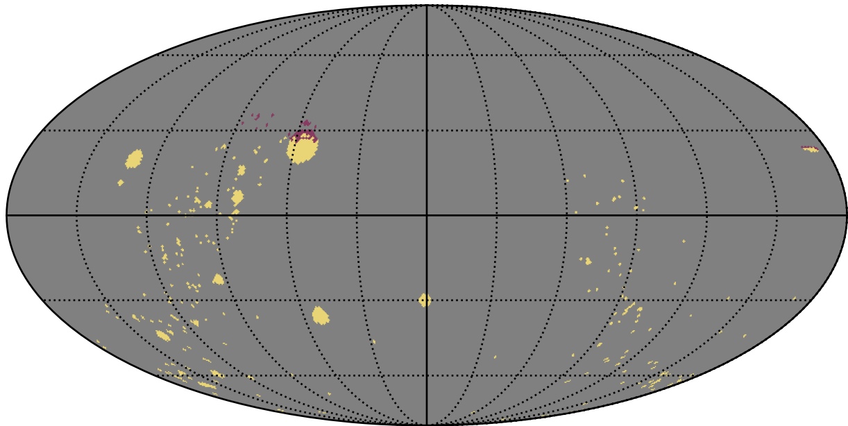
weather_cloudso6v3.4_10yrs : GalplaneFootprintMetric_open_clusters_map_Tau_73_0
