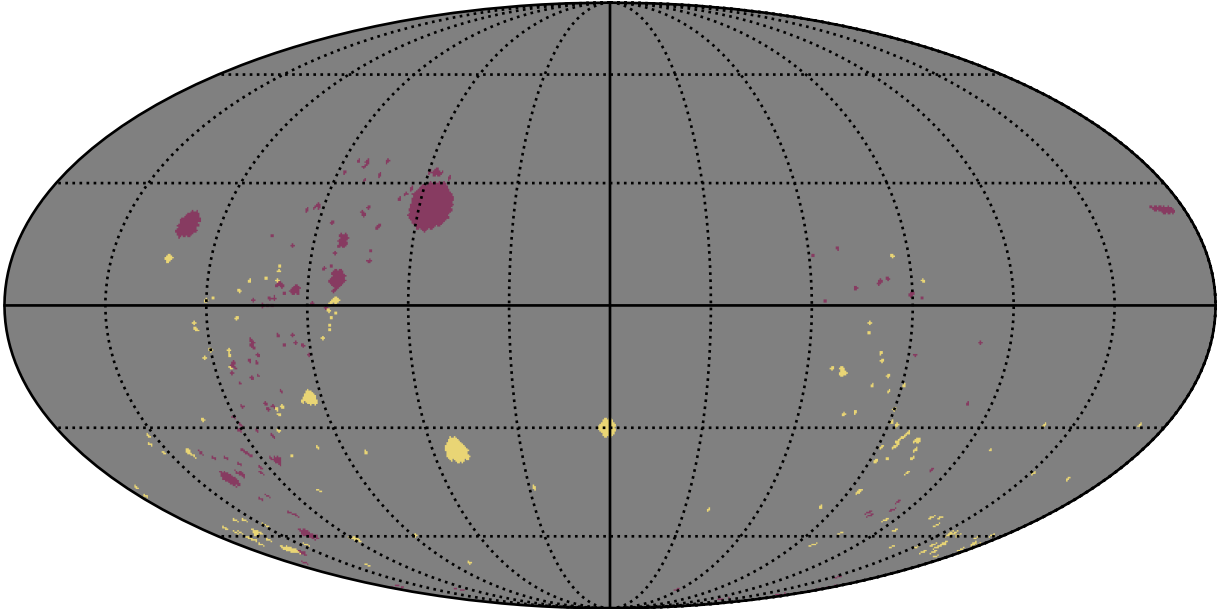
weather_cloudso6v3.4_10yrs : GalplaneFootprintMetric_open_clusters_map_Tau_11_0
