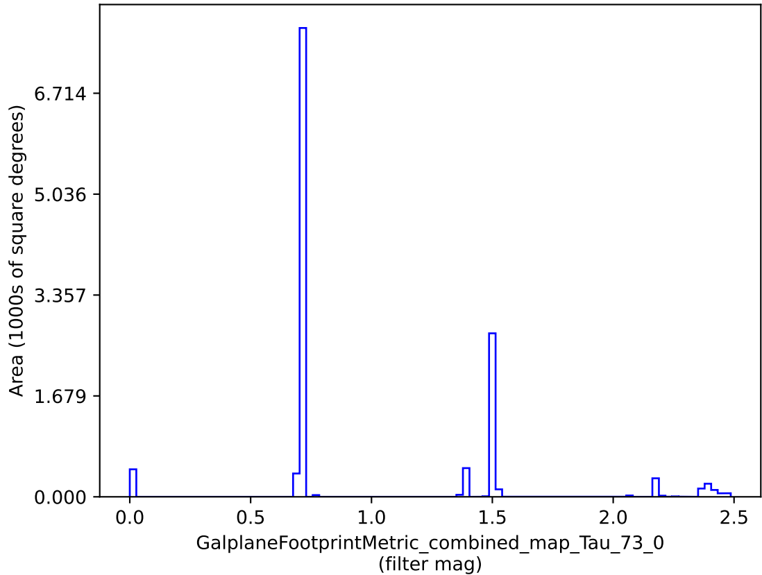
weather_cloudso6v3.4_10yrs : GalplaneFootprintMetric_combined_map_Tau_73_0
