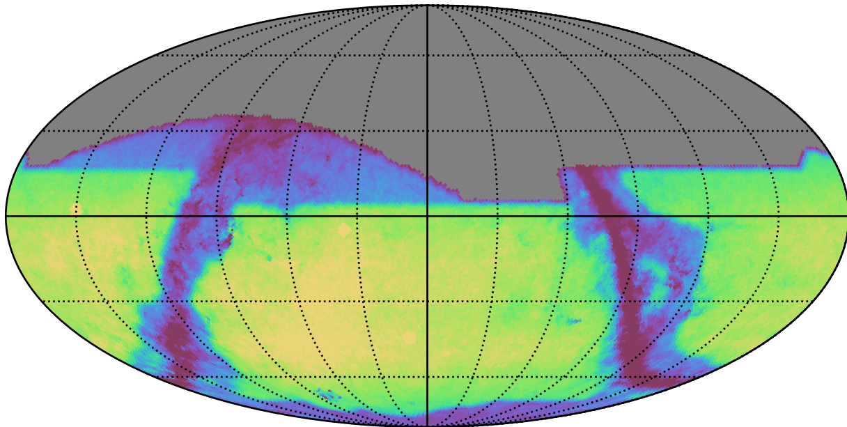
weather_cloudso6v3.4_10yrs z: GalaxyCountsMetricExtended
