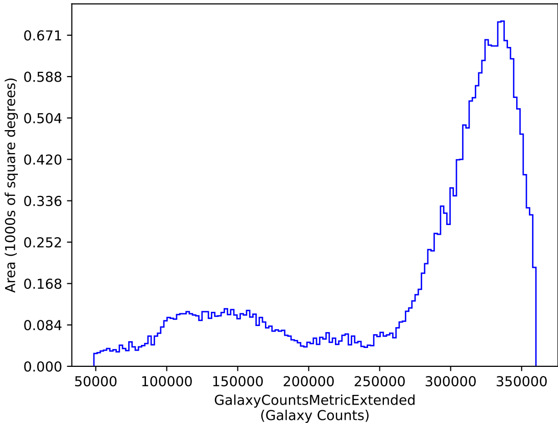
weather_cloudso6v3.4_10yrs y: GalaxyCountsMetricExtended
