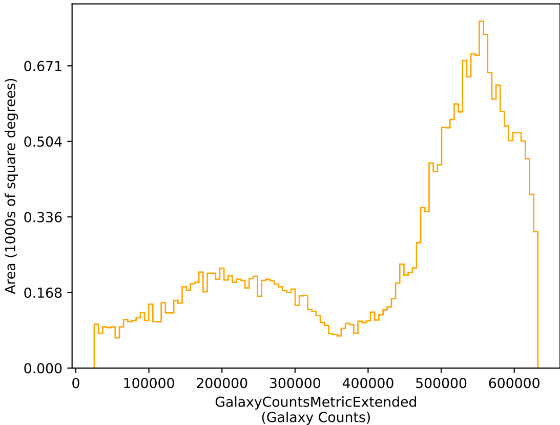
weather_cloudso6v3.4_10yrs r: GalaxyCountsMetricExtended
