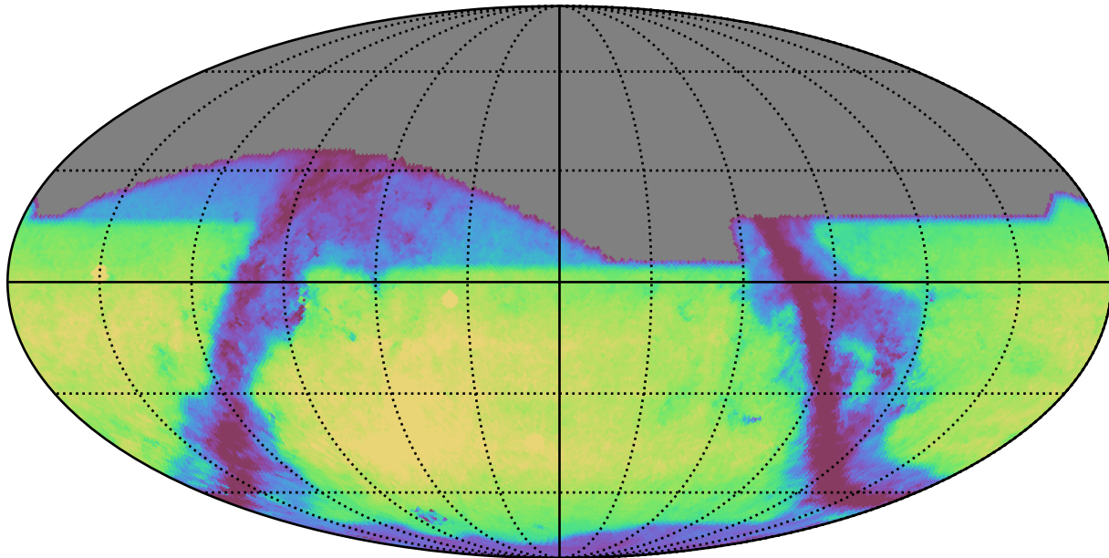
weather_cloudso6v3.4_10yrs i: GalaxyCountsMetricExtended
