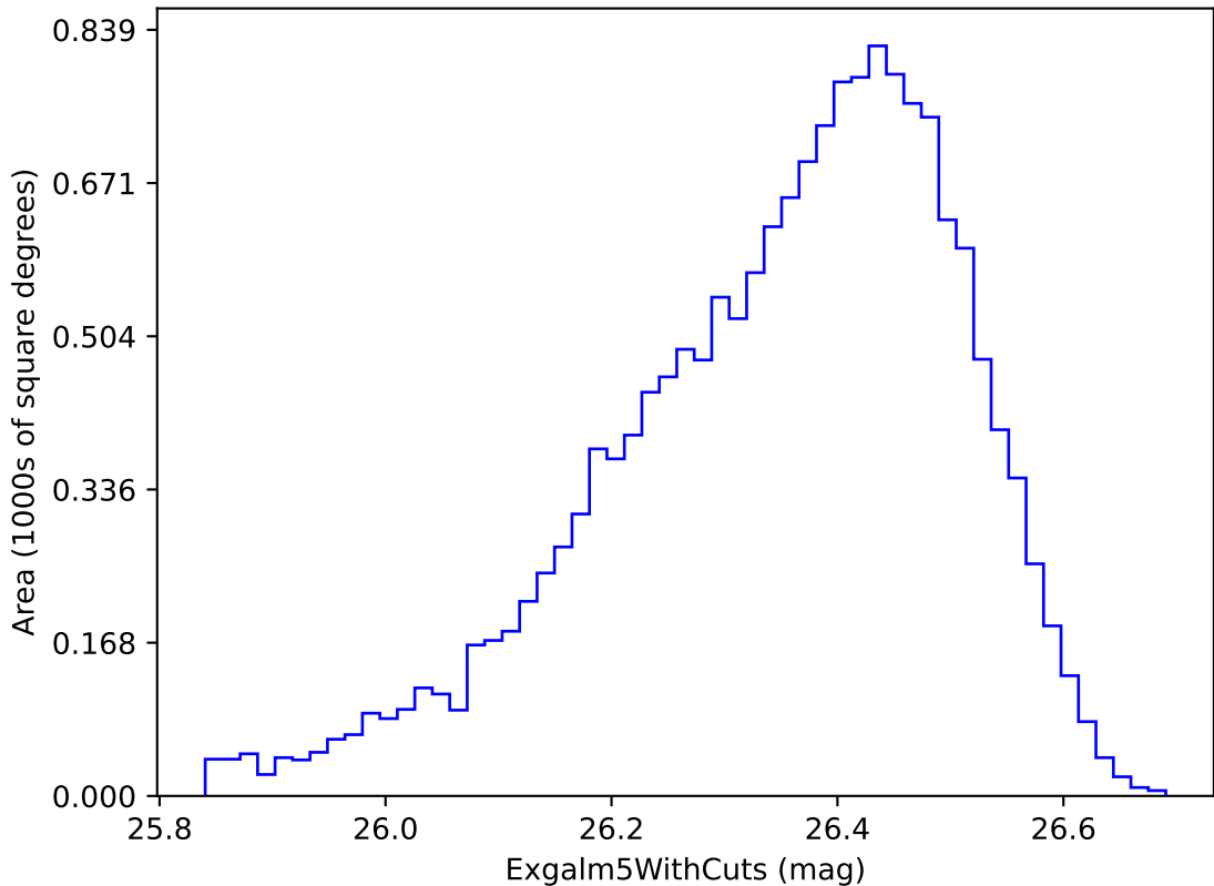
weather_cloudso6v3.4_10yrs i band non-DD year 9: Exgalml5WithCuts
