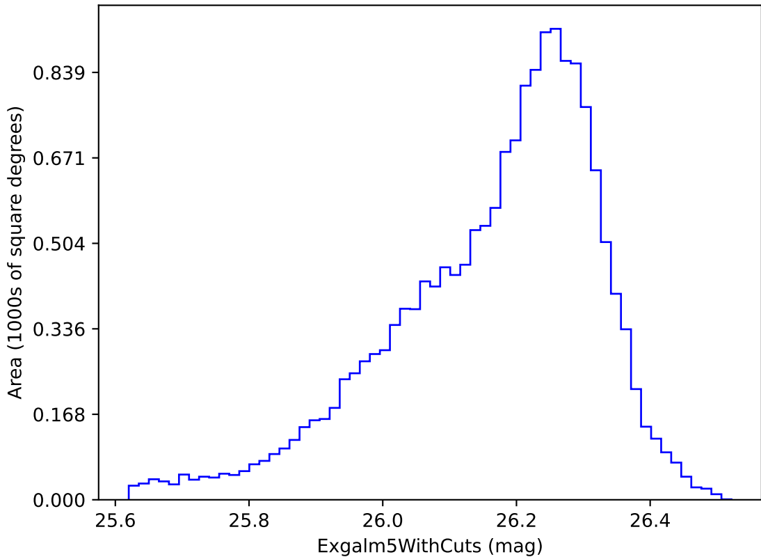
weather_cloudso6v3.4_10yrs i band non-DD year 6: Exgalml5WithCuts
