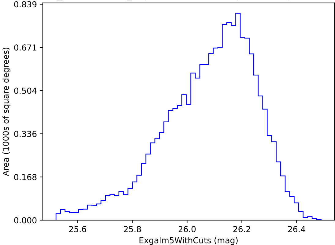
weather_cloudso6v3.4_10yrs i band non-DD year 5: Exgalml5WithCuts
