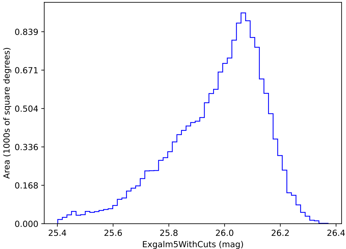
weather_cloudso6v3.4_10yrs i band non-DD year 4: Exgalm5WithCuts
