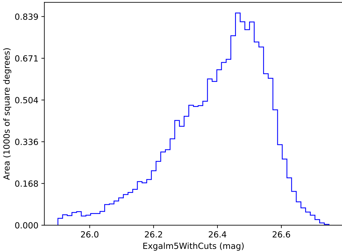
weather_cloudso6v3.4_10yrs i band non-DD year 10: ExgalM5WithCuts
