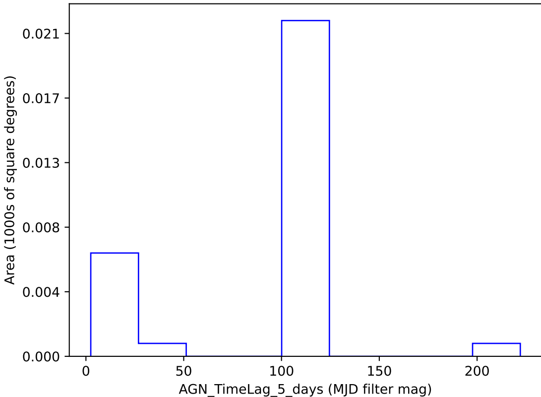
weather_cloudso6v3.4_10yrs y band: AGN_TimeLag_5_days
