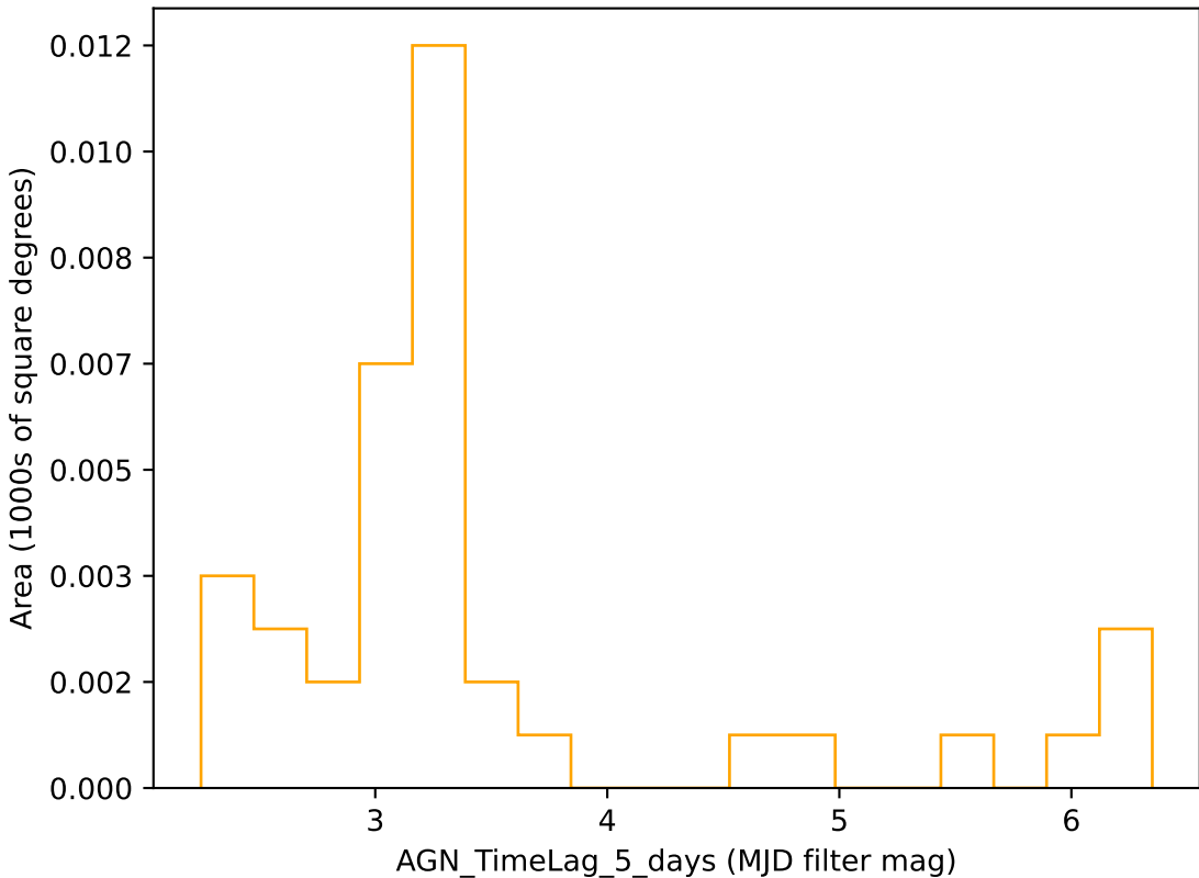
weather_cloudso6v3.4_10yrs r band: AGN_TimeLag_5_days
