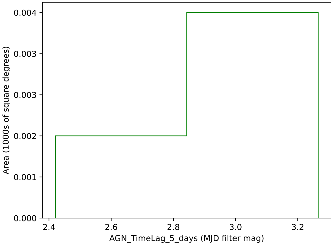
weather_cloudso6v3.4_10yrs g band: AGN_TimeLag_5_days
