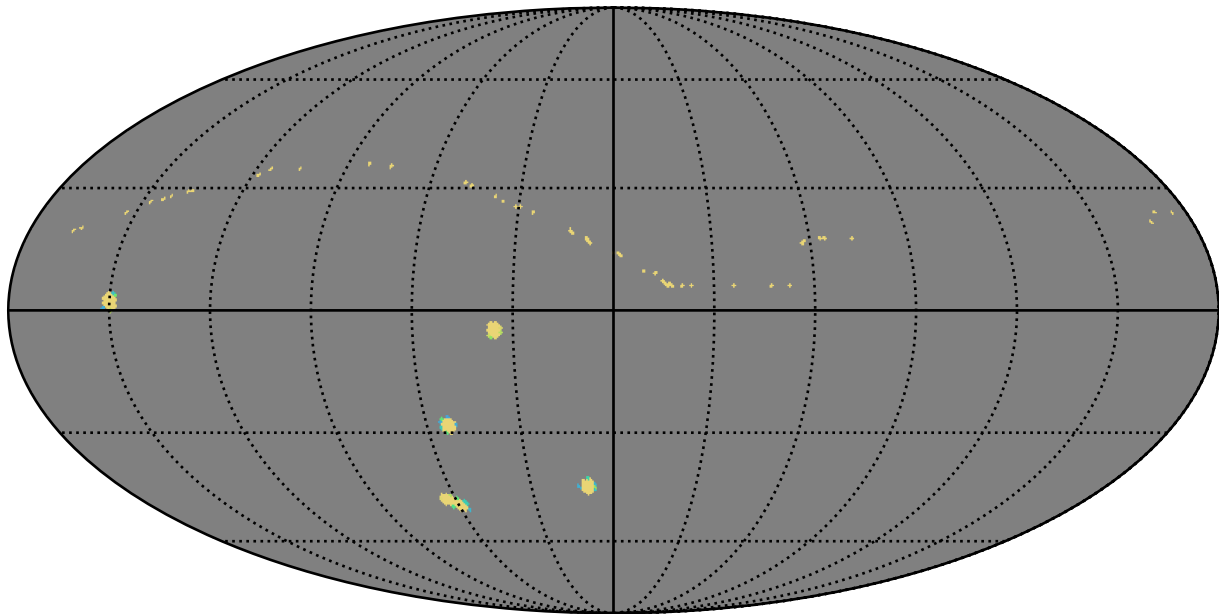
weather_cloudso6v3.4_10yrs all bands: AGN_TimeLag_5_days
