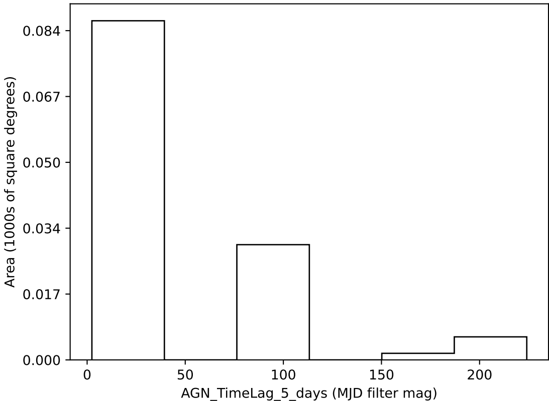
weather_cloudso6v3.4_10yrs all bands: AGN_TimeLag_5_days
