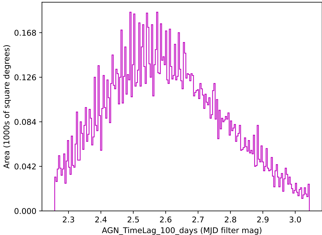
weather_cloudso6v3.4_10yrs z band: AGN_TimeLag_100_days
