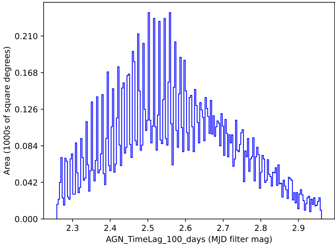
weather_cloudso6v3.4_10yrs y band: AGN_TimeLag_100_days
