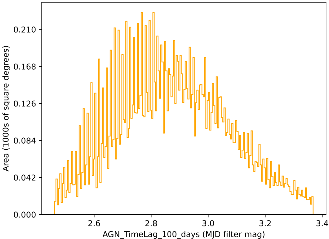
weather_cloudso6v3.4_10yrs r band: AGN_TimeLag_100_days
