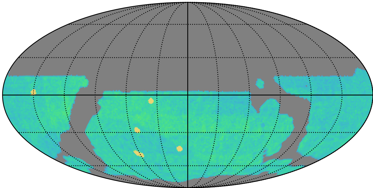
weather_cloudso6v3.4_10yrs i band: AGN_TimeLag_100_days
