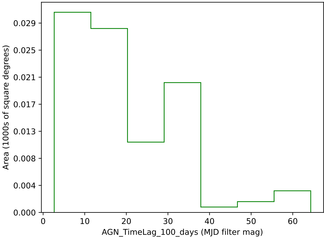
weather_cloudso6v3.4_10yrs g band: AGN_TimeLag_100_days
