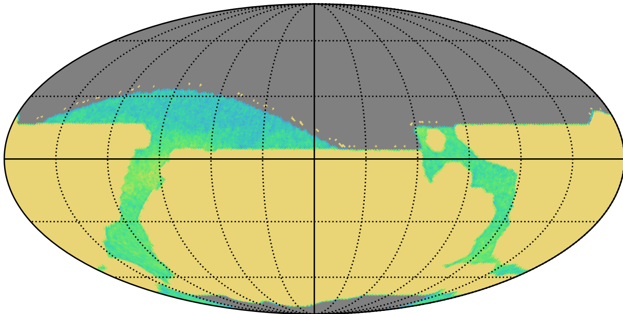
weather_cloudso6v3.4_10yrs all bands: AGN_TimeLag_100_days
