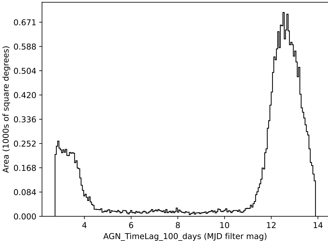
weather_cloudso6v3.4_10yrs all bands: AGN_TimeLag_100_days
