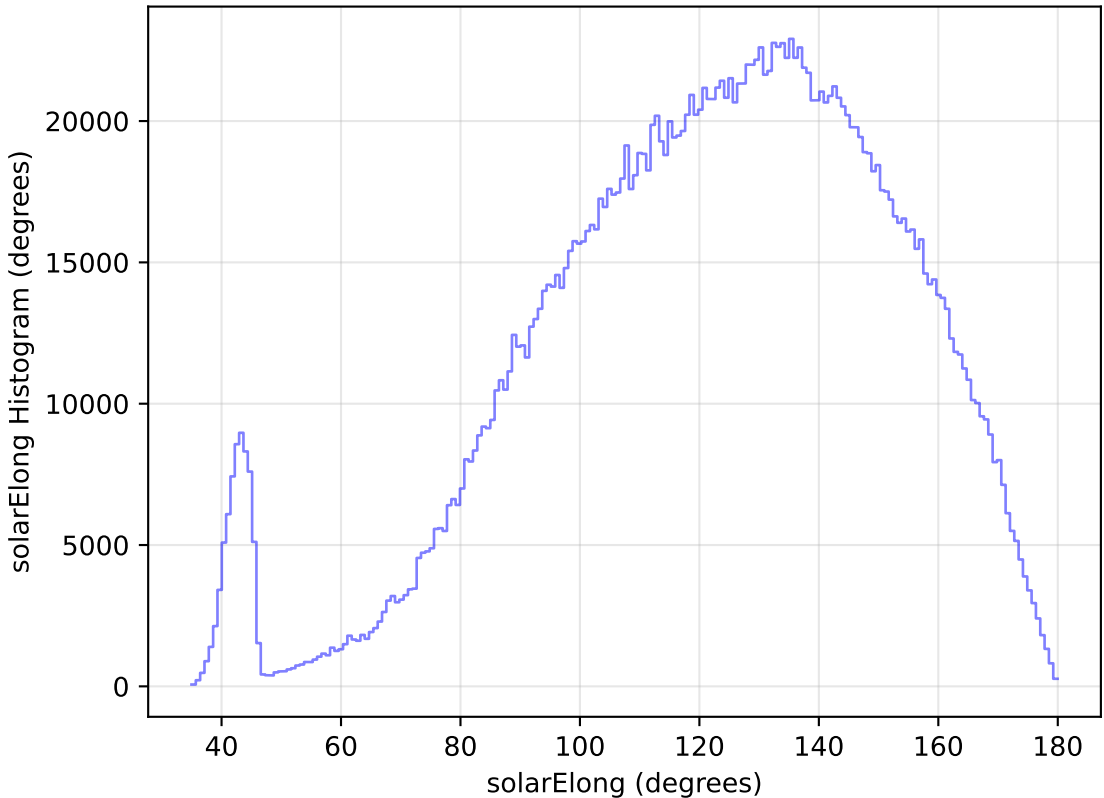
weather_cloudso6v3.4_10yrs WFD all bands: solarElong Histogram
