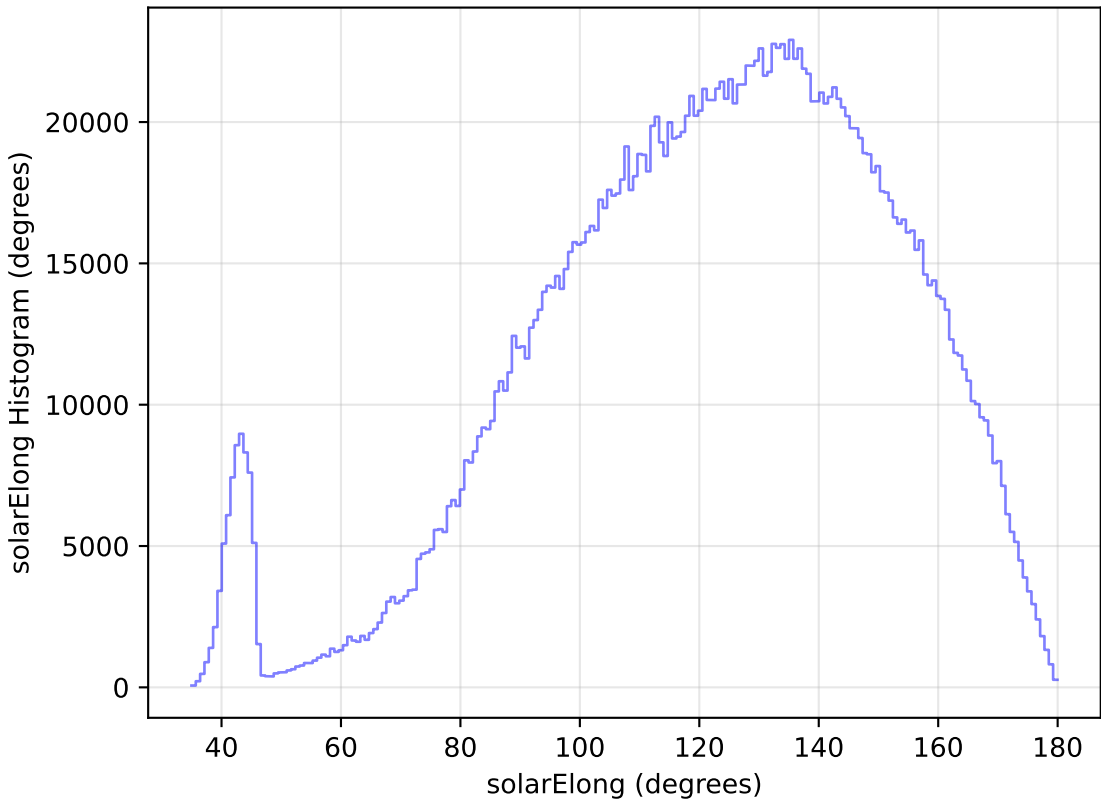
weather_cloudso6v3.4_10yrs All sky all bands: solarElong Histogram
