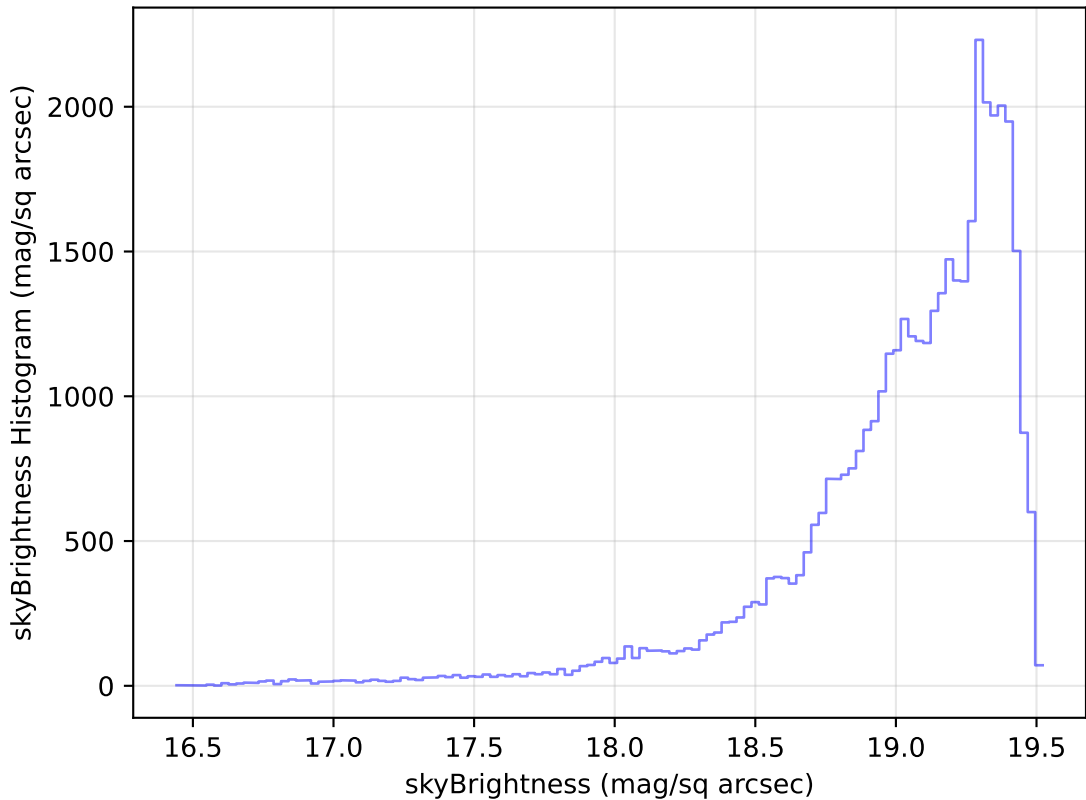
weather_cloudso6v3.4_10yrs Yr 1 z band: skyBrightness Histogram
