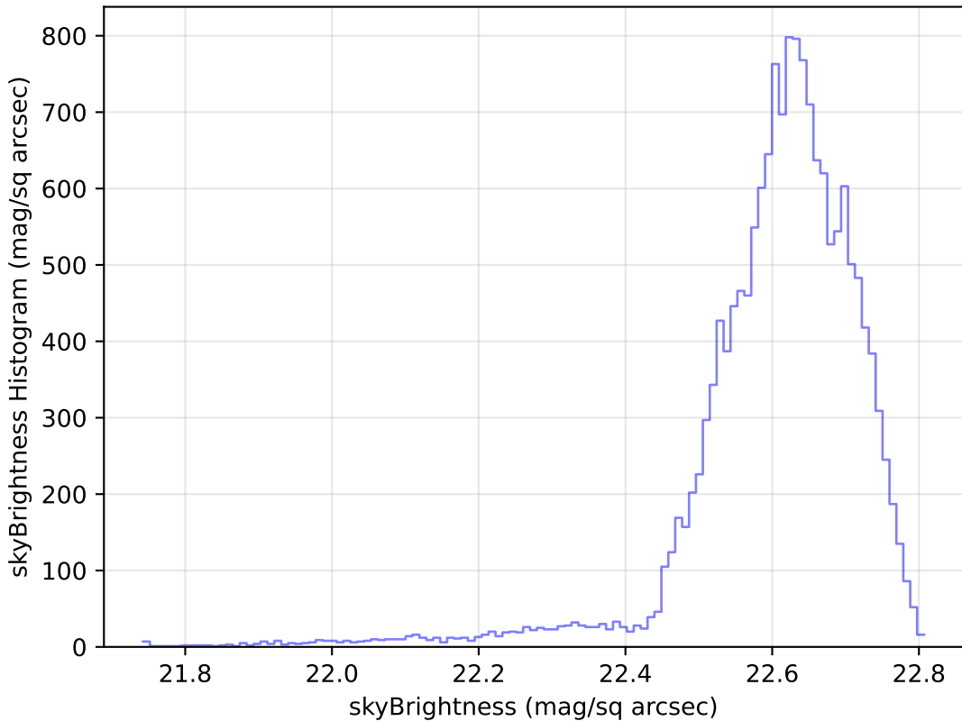
weather_cloudso6v3.4_10yrs Yr 1 u band: skyBrightness Histogram
