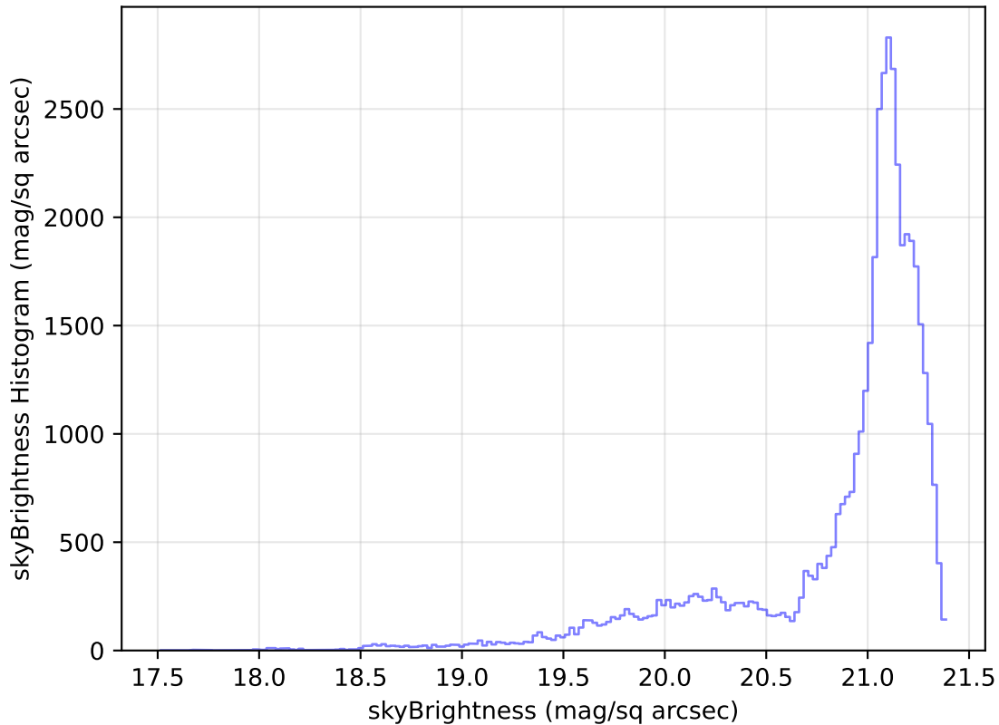
weather_cloudso6v3.4_10yrs Yr 1 r band: skyBrightness Histogram
