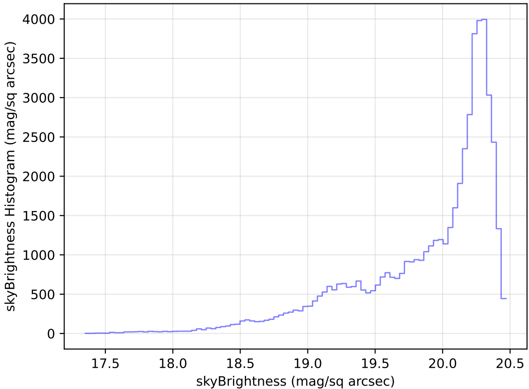
weather_cloudso6v3.4_10yrs Yr 1 i band: skyBrightness Histogram
