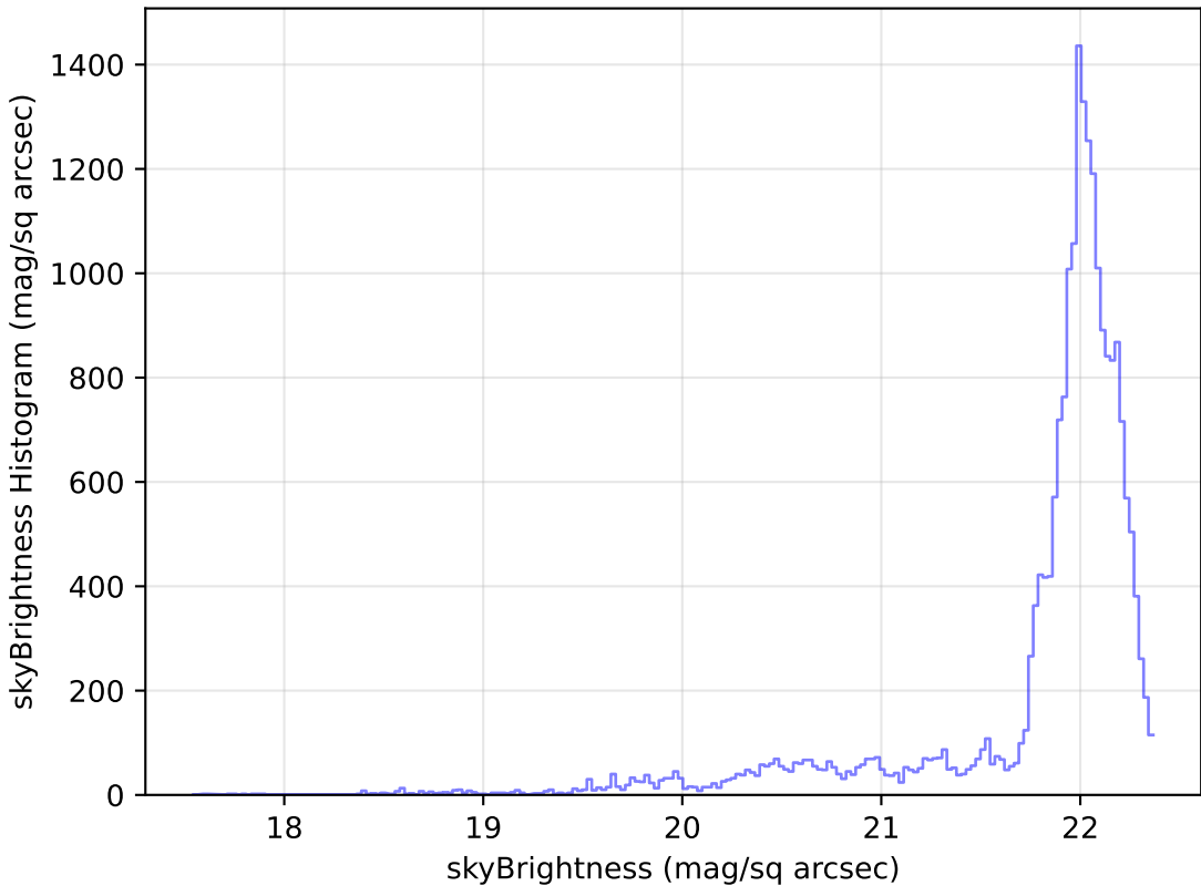
weather_cloudso6v3.4_10yrs Yr 1 g band: skyBrightness Histogram
