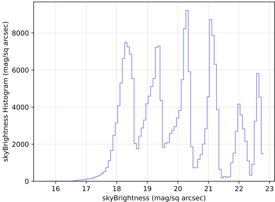
weather_cloudso6v3.4_10yrs Yr 1 all bands: skyBrightness Histogram
