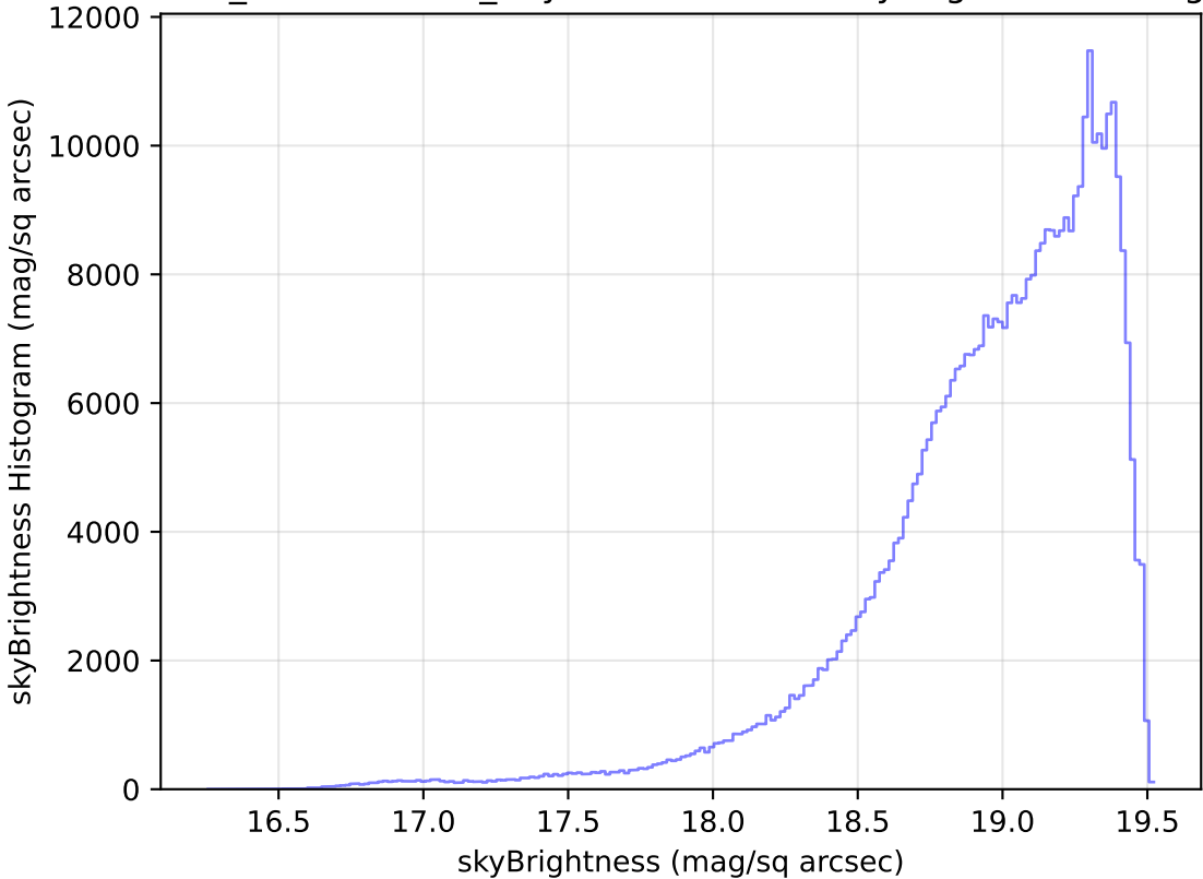
weather_cloudso6v3.4_10yrs WFD z band: skyBrightness Histogram
