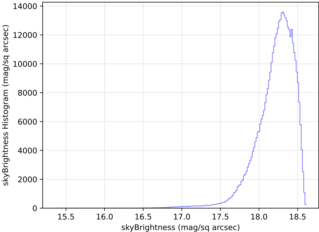
weather_cloudso6v3.4_10yrs WFD y band: skyBrightness Histogram
