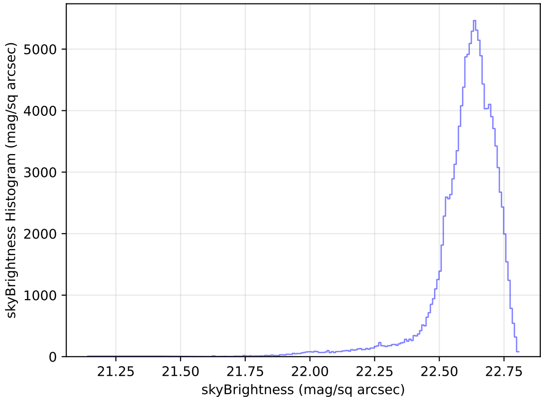
weather_cloudso6v3.4_10yrs WFD u band: skyBrightness Histogram
