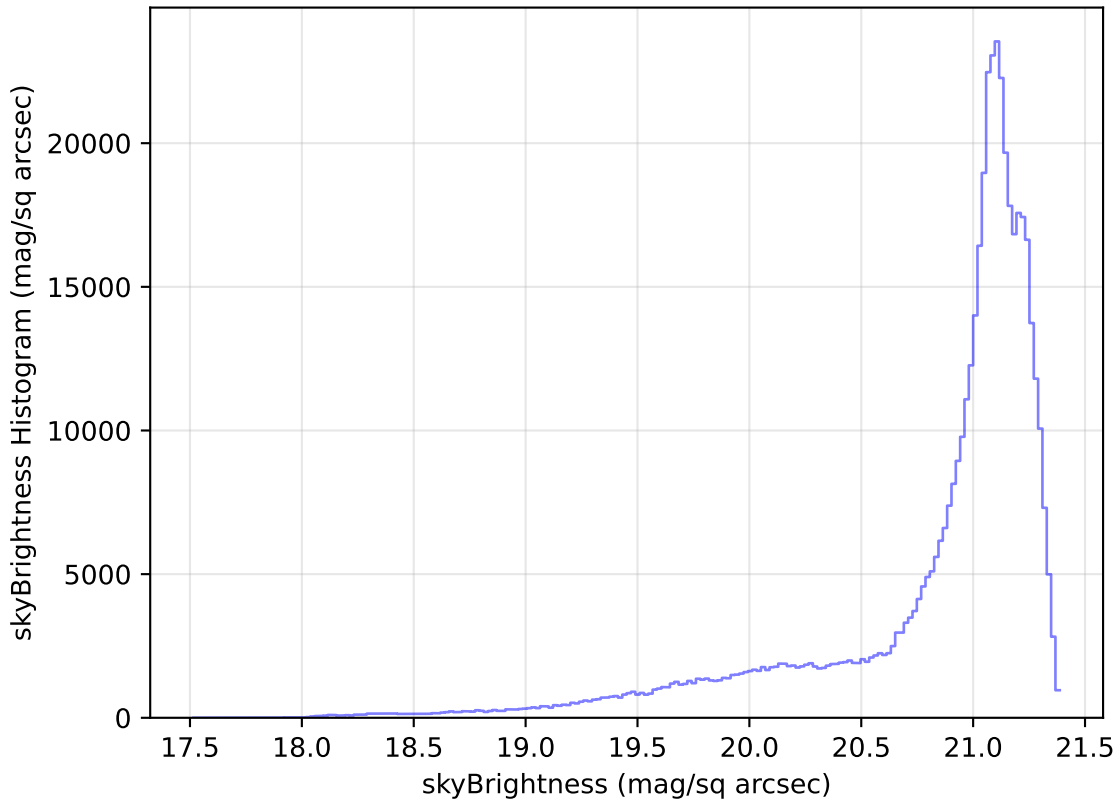
weather_cloudso6v3.4_10yrs WFD r band: skyBrightness Histogram
