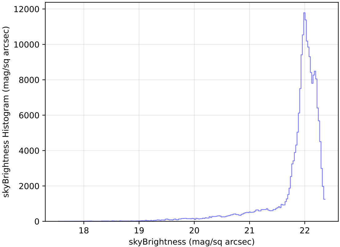
weather_cloudso6v3.4_10yrs WFD g band: skyBrightness Histogram
