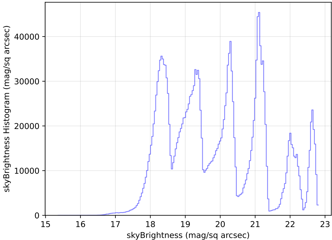
weather_cloudso6v3.4_10yrs WFD all bands: skyBrightness Histogram
