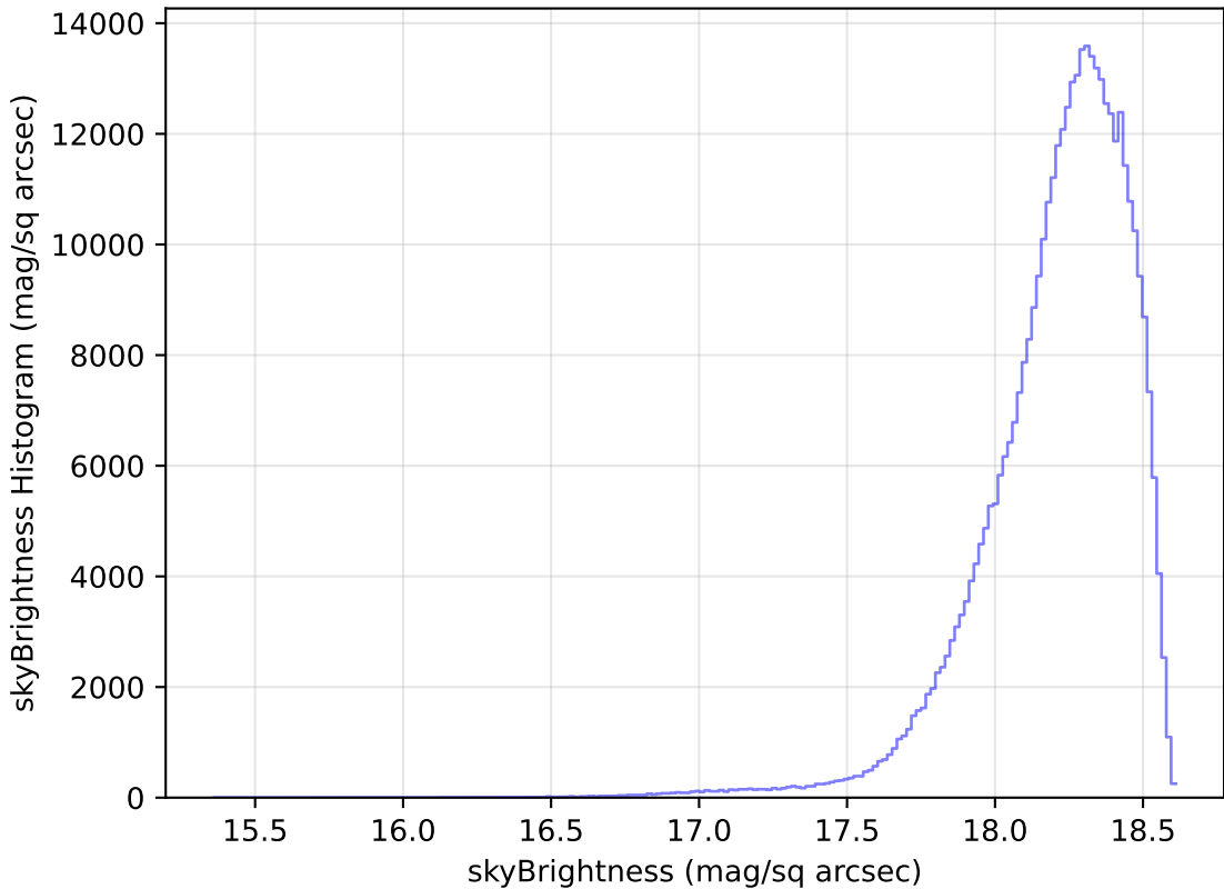
weather_cloudso6v3.4_10yrs All sky y band: skyBrightness Histogram
