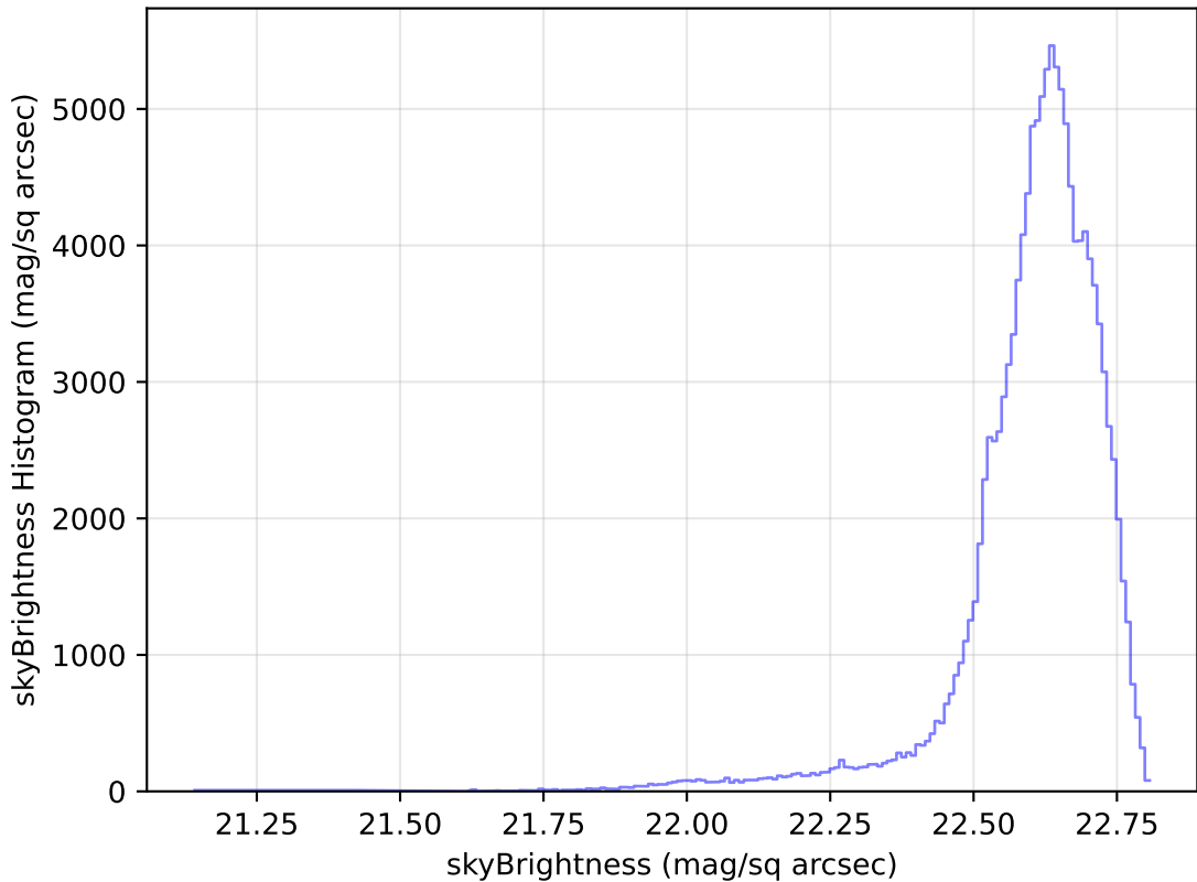
weather_cloudso6v3.4_10yrs All sky u band: skyBrightness Histogram
