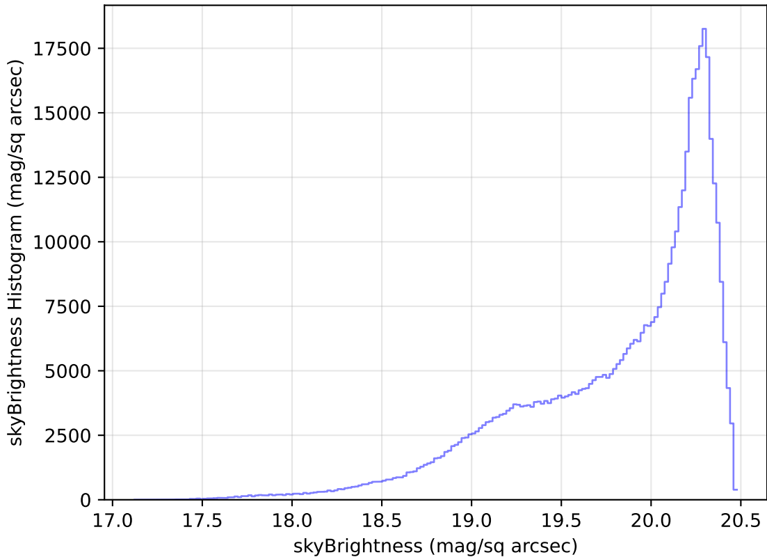
weather_cloudso6v3.4_10yrs All sky i band: skyBrightness Histogram
