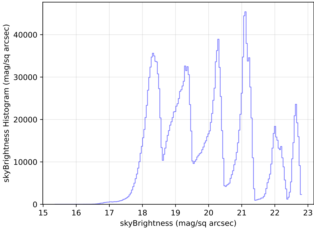
weather_cloudso6v3.4_10yrs All sky all bands: skyBrightness Histogram
